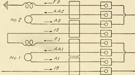
Fig. 55. Forward Position of Reverse
